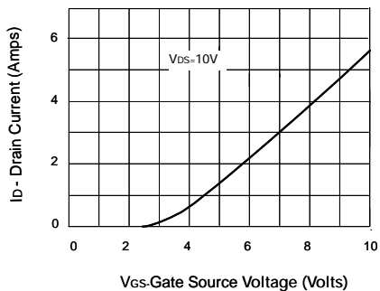
Transfer Characteristics
